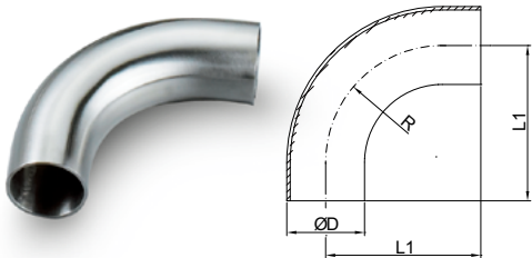
90°焊接式弯头长型 90° Welded Elbow (Long Type)
