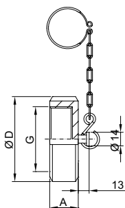
带链条盲螺母 Blind Cap with Chain
