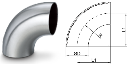
90°焊接式弯头 90° Welded Elbow
