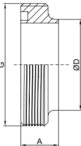
带链条盲螺母 Blind Cap with Chain
