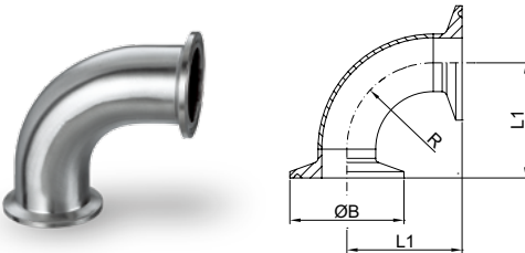
90°卡箍式弯头 90° Clamped Elbow
