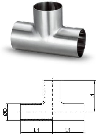
焊接式三通 Welded Tee
