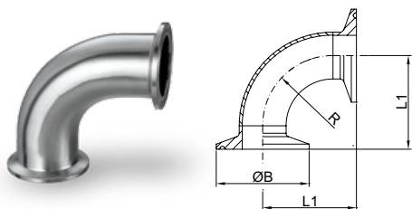
90°卡箍式弯头 90° Clamped Elbow
